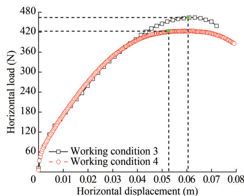
Figure 9 Horizontal load–displacement curves at different loading speeds
