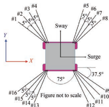
Figure 2 Schematic layout of the mooring system
