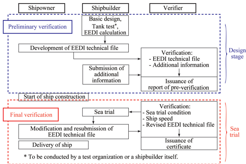
Figure 2 Overall process of EEDI verification (IMO, 2016b)
