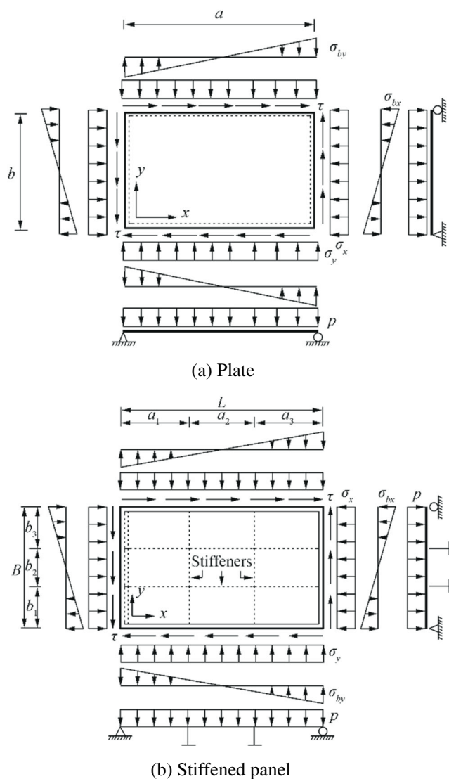
Figure 13 Application of combined in-plane and out-of-plane loads
