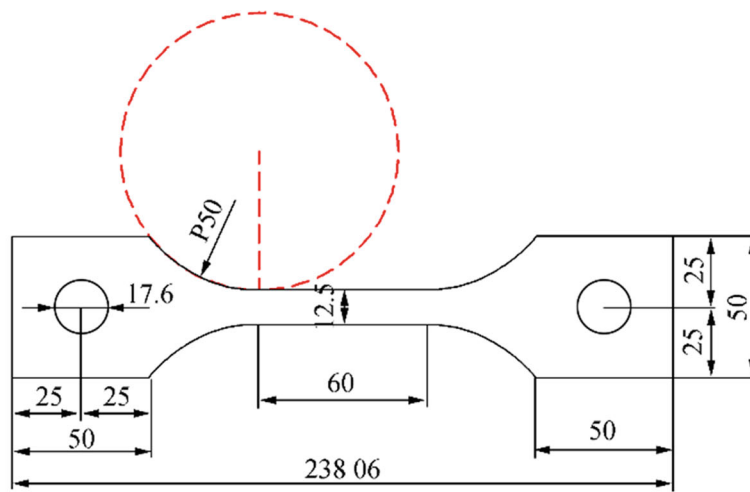
(a) Dimension of the tensile test specimen
