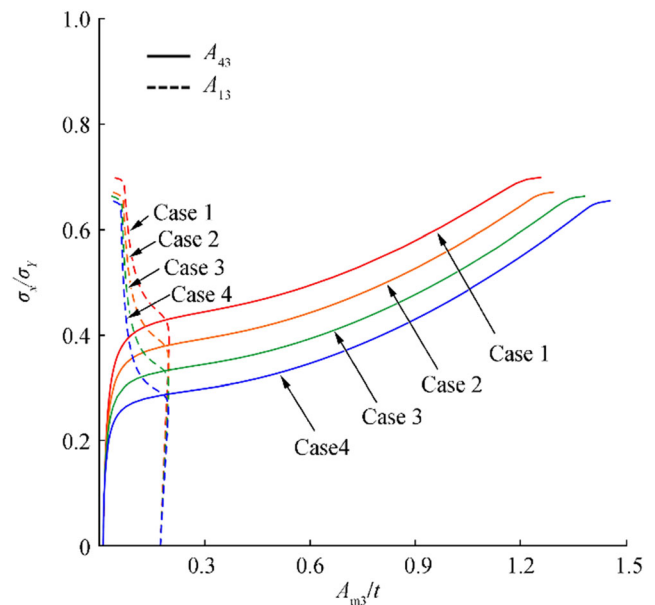
Figure 24 The ALPS/SPINE ultimate compressive strength behavior of the plate panel in terms of the added deflection components
