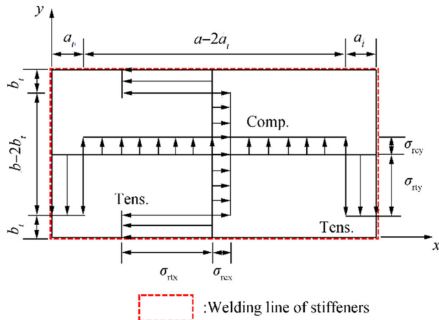
Figure 11 Idealization of the welding-induced residual stresses in a plate
