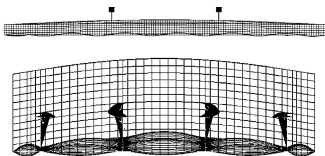
Figure 17 Modeling of initial deformations in the plate and support members
