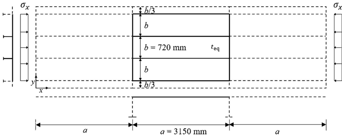
Figure 12 Extent of the ALPS/ULSAP and ALPS/SPINE analyses
