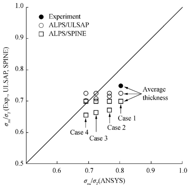
Figure 25 Comparison of the ultimate compressive strength between the analyses and the experiment for the plate panel with varying the thickness
