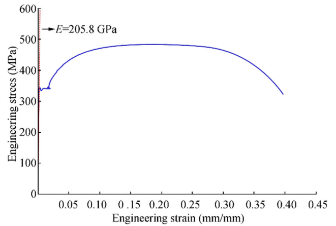
Figure 4 Engineering stress versus engineering strain curve of the AH32 steel
