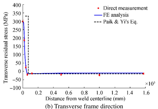
Figure 10 A comparison of welding-induced residual stresses between direct measurements, numerical predictions, and simple formula estimations
