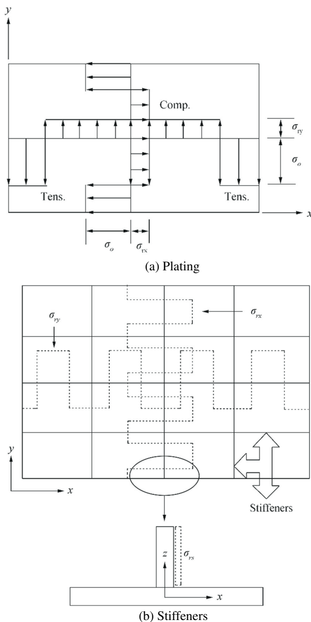
Figure 14 Idealized welding-induced residual stress distributions
