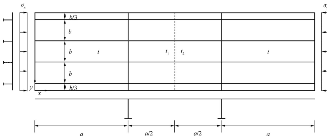
Figure 1 A stiffened plate panel
