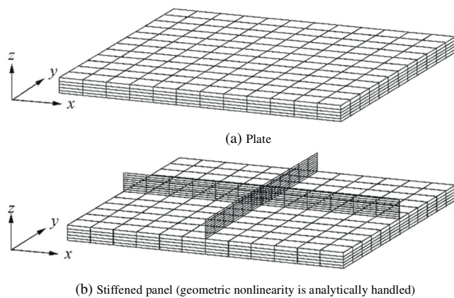
Figure 15 Example subdivision of mesh regions used for treatment of plasticity
