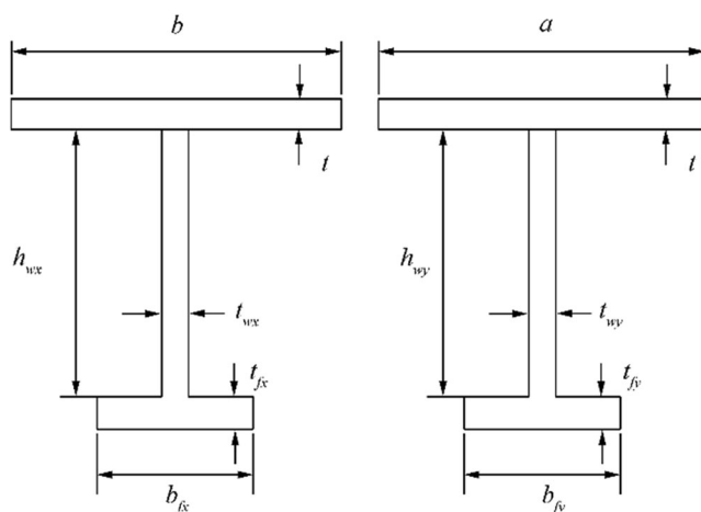
Figure 2 T-type support members in the x and y directions
