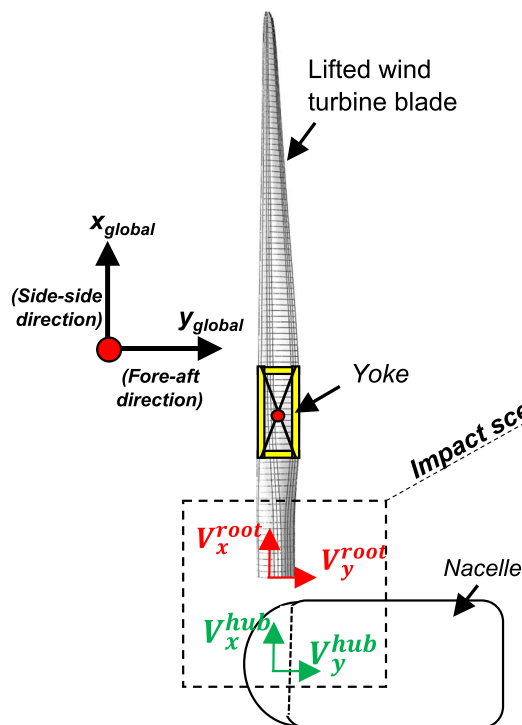
Figure 3 Illustration of impact scenarios during the blade mating process
