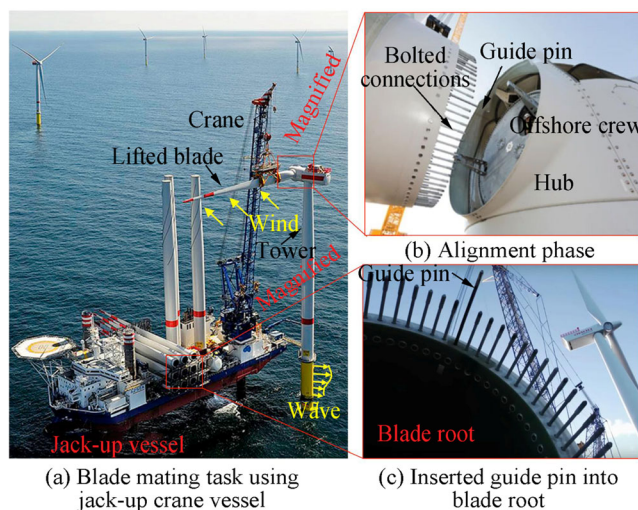
Figure 1 Blade root mating process ( https://orsted.com/en ) ( https://vessels.offshorewind.biz/vessels/sea_challenger ) ( https://www.siemens.com )
