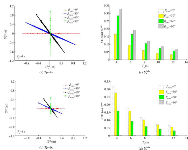
Figure 11 Motion of hub-centre in xy -plane and comparison of standard deviations for load case H_s = 2.5 \text{ m} , T_p = 4 \text{ s}, 6 \text{ s}, 8 \text{ s}, 10 \text{ s}, 12 \text{ s} , U_w = 10 \text{ m/s} and \beta_{\text{wave}} = 0^\circ, 30^\circ, 60^\circ and 90^\circ
