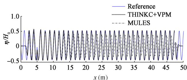
Figure 2 2D wave simulation results interFOAM vs. THINC + VPM (Zhang et al. 2019)
