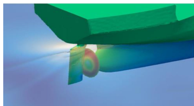
(a) Dynamic pressure at the stern
