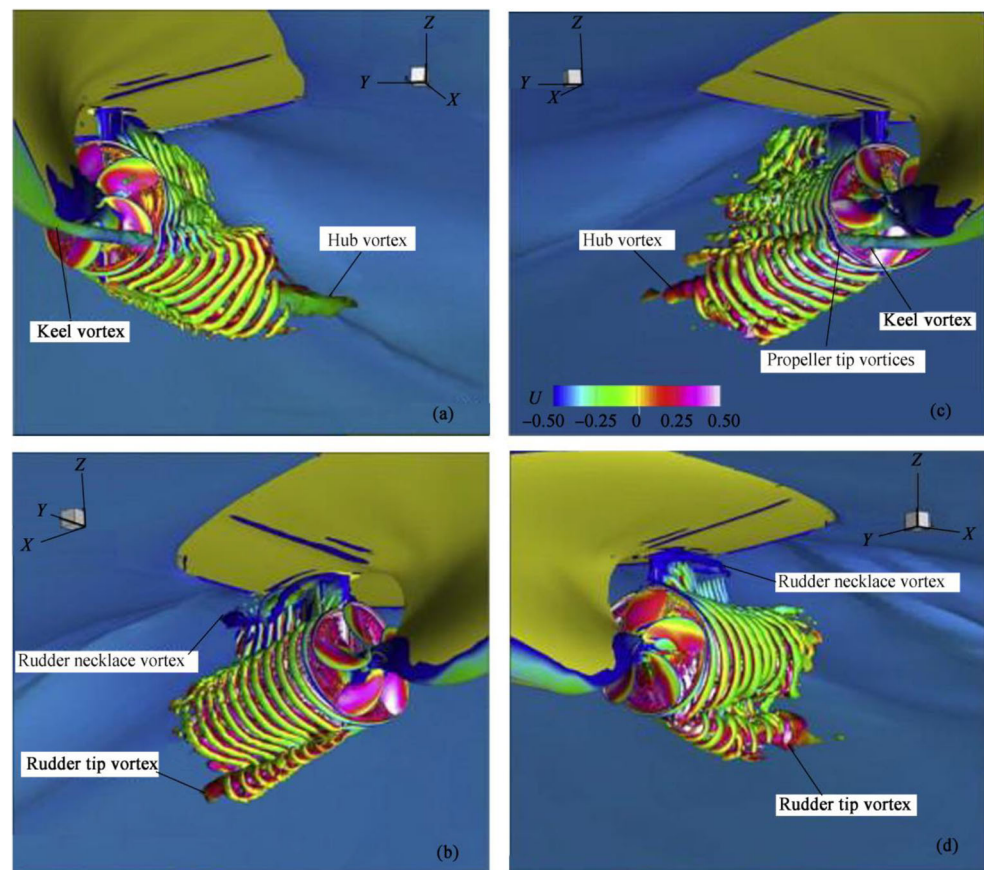
Figure 6 Isosurfaces of Q = 5000 colored with dimensionless U -velocity for the 15/1 maneuver. a and c show zero yaw, and b and d are maximum and minimum yaw, respectively (Mofidi and Carrica 2014)
