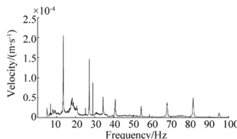
Fig. 14 Velocity spectrum measured in measurement point 40
