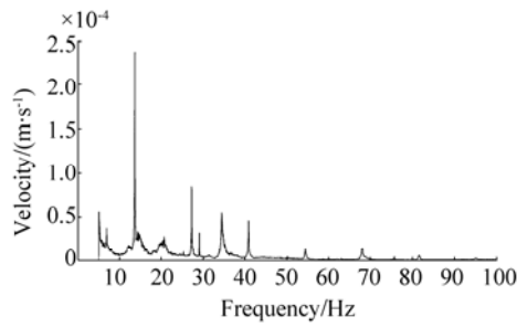
Fig. 15 Velocity spectrum measured in measurement point 101
