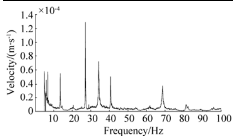
Fig. 13 Velocity spectrum measured in measurement point 35
